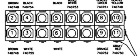
DETAIL 1 DETAIL FOR WIRE LOCATIONS FROM SWITCH PLATE REAR VIEW OF TERMINAL HOUSING
