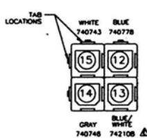
DETAIL 5 DETAIL FOR WIRE LOCATIONS FROM VAC AND PUMP CONTROLS REAR VIEW OF TERMINAL HOUSING
