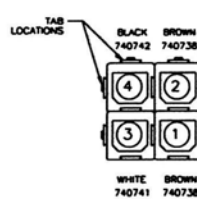
DETAIL 3 DETAIL FOR WIRE LOCATIONS FROM SPEED/MAIN CONTROLS AND VAC/PUMP CONTROLS REAR VIEW OF TERMINAL HOUSING
